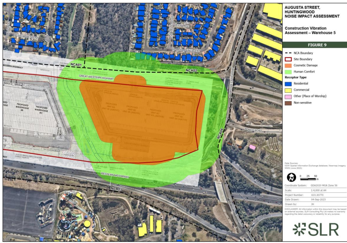
Figure 9 Construction Vibration Assessment – Building 5
