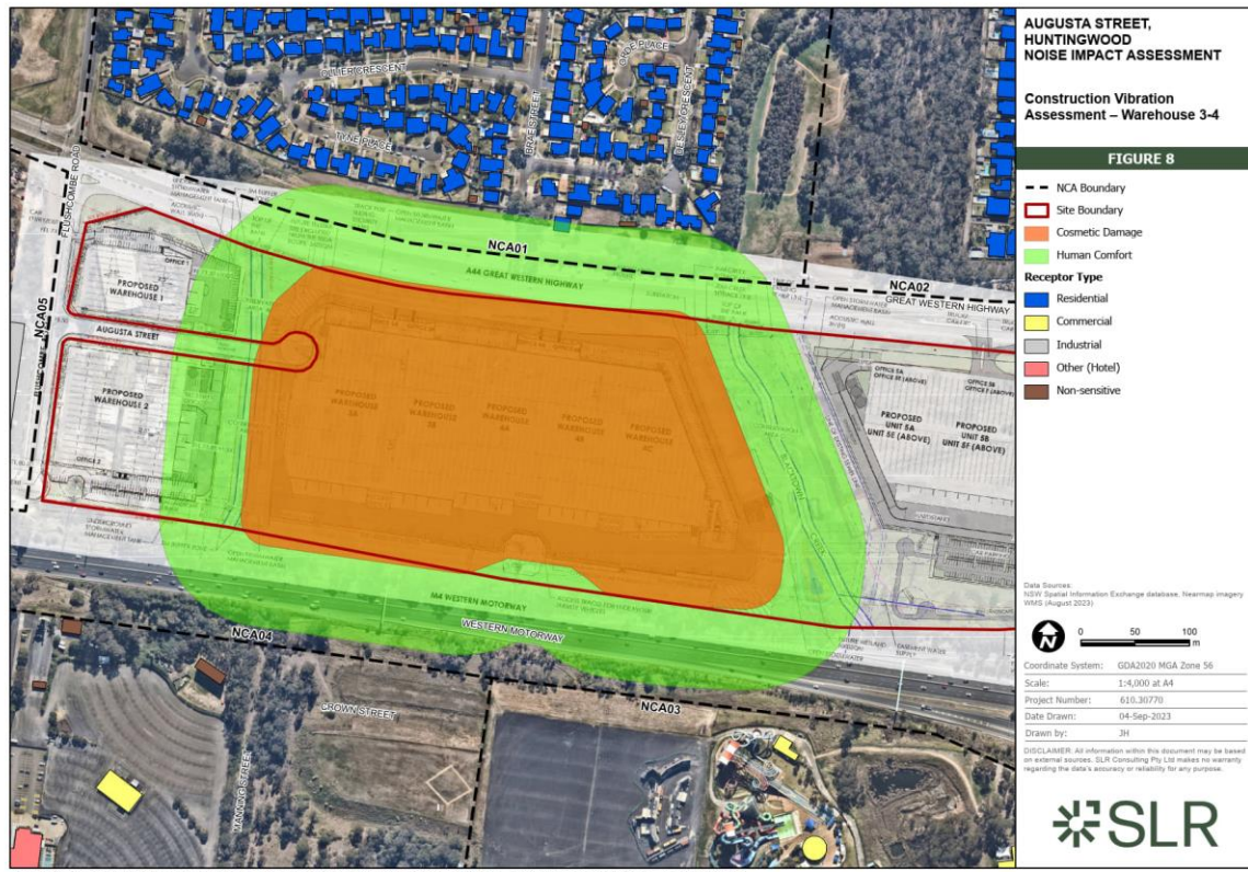
Figure 8 Construction Vibration Assessment – Building 3-4
