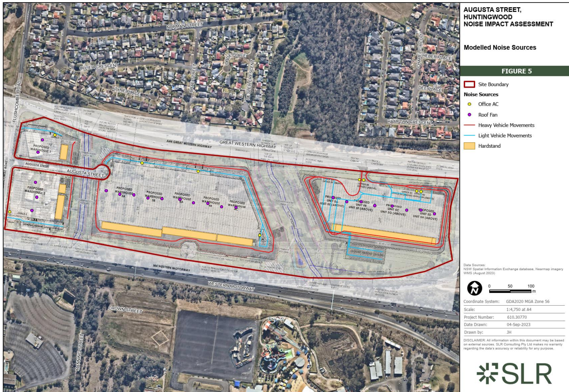
Figure 5 Modelled Noise Sources
