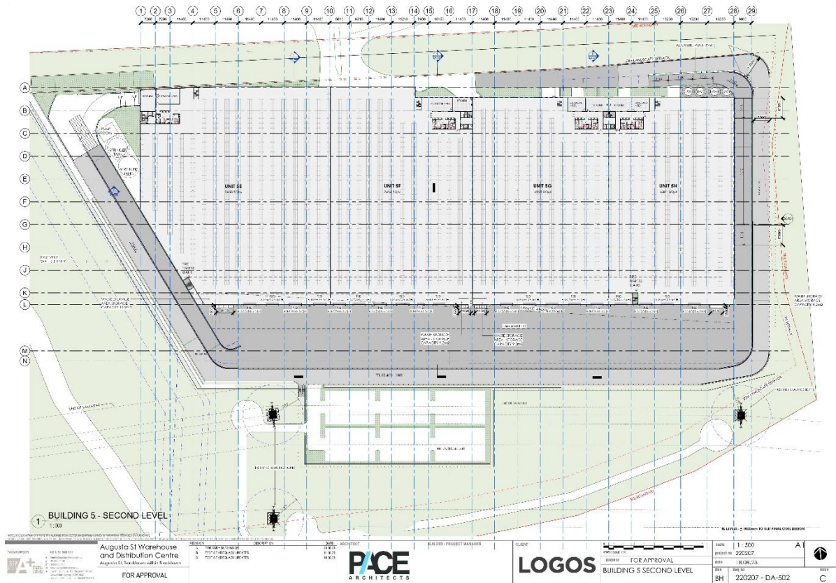
Figure 4 Proposed Development – Second Floor
