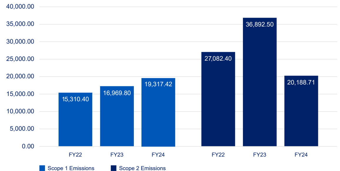
Global Greenhouse Gas Emissions FY22-FY24 (Metric Tons of CO2e)
