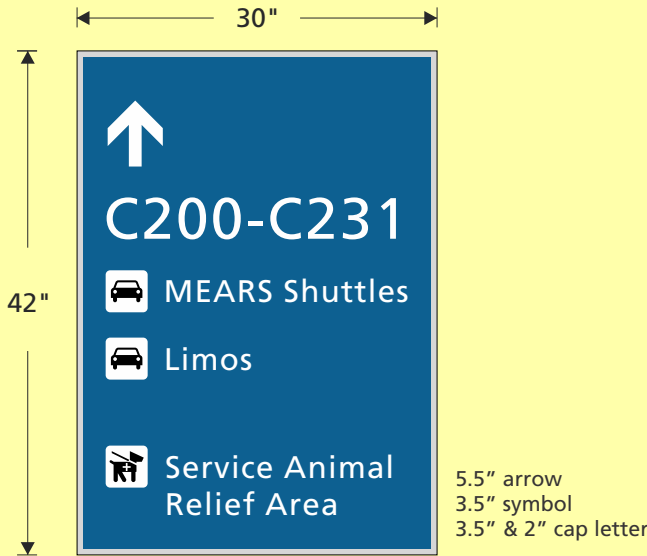
6 Graphic View Scale is 3/4" = 1'
