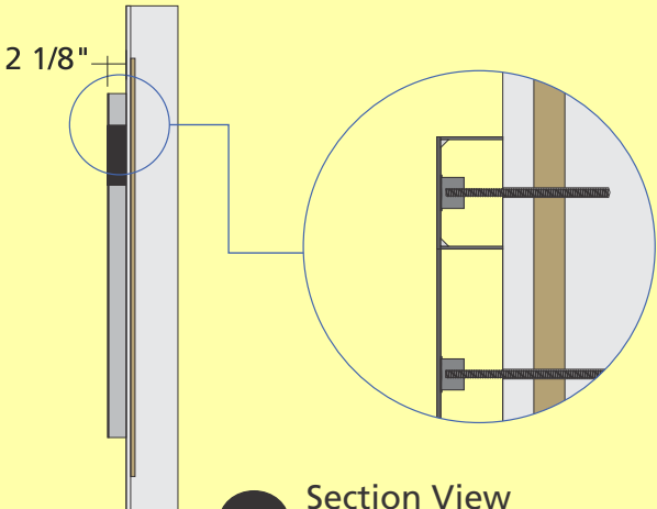
73.2 Section View Not to Scale
