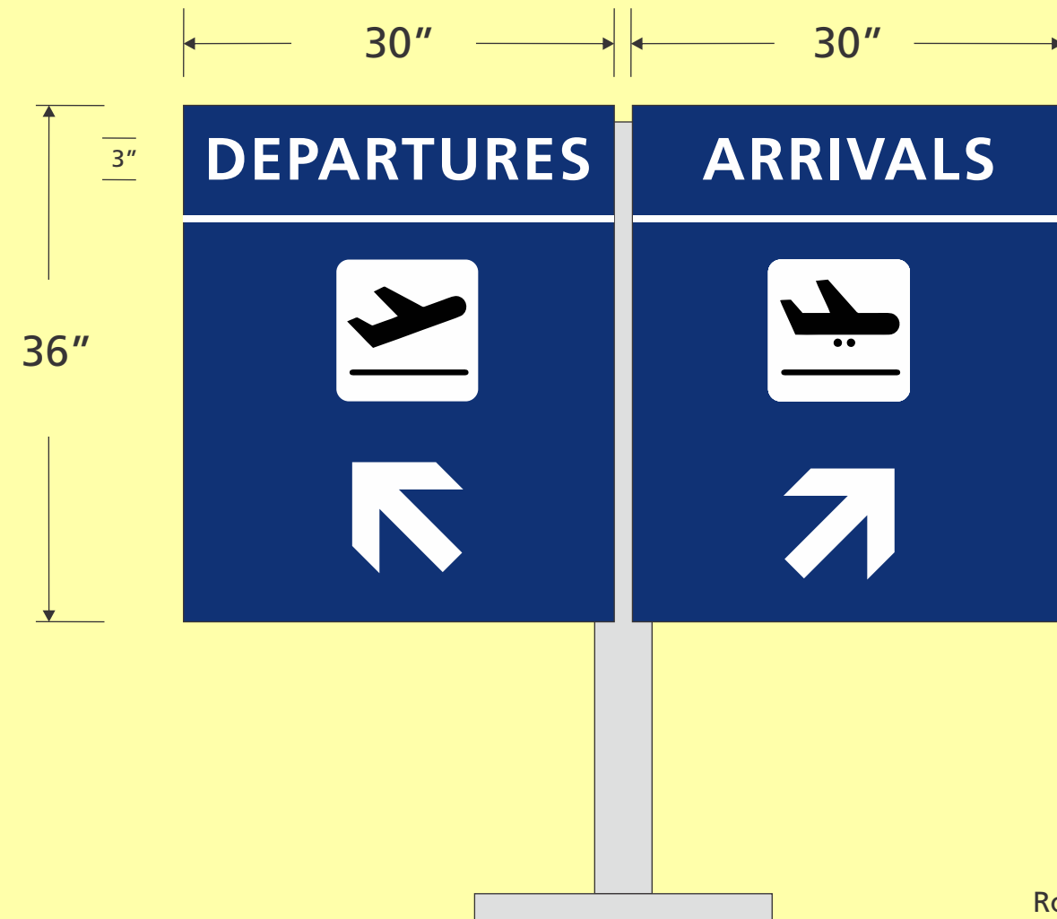
65.1 Graphic View Scale is 1" = 1'
