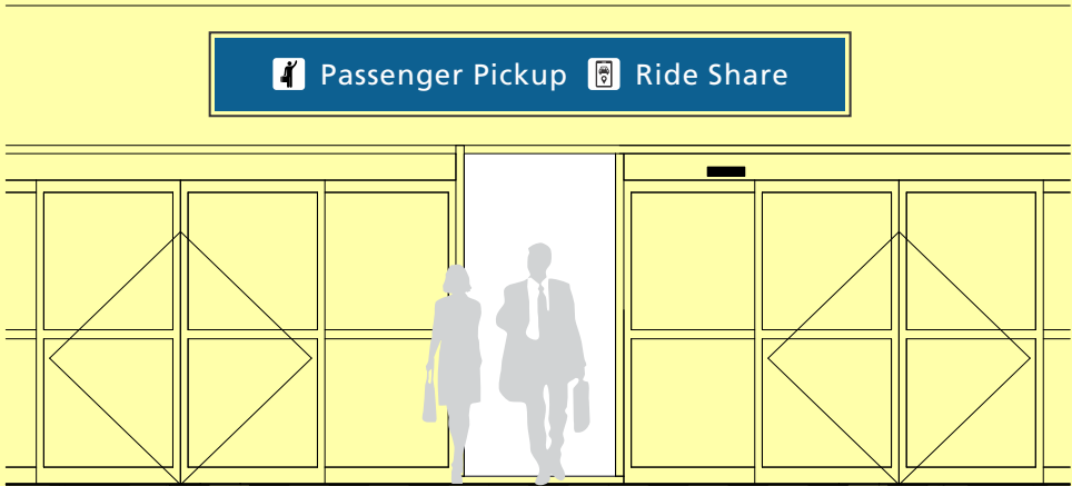
17 Elevation View (ride share exits) Not to Scale
