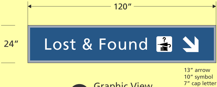
5.1 Graphic View Scale is 3/8" = 1'
