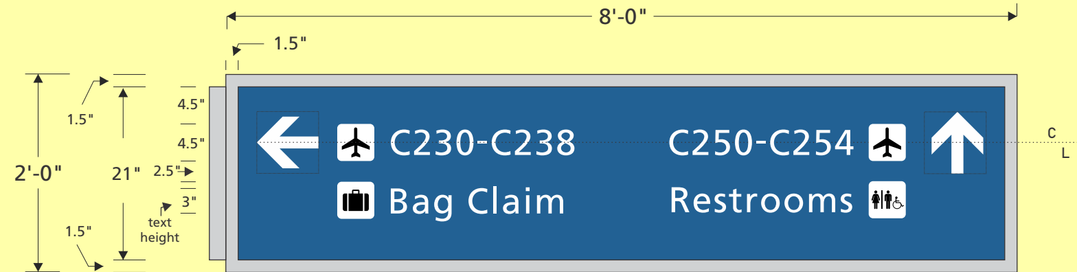
34 Graphic View (side A) Scale is 3/4" = 1'
