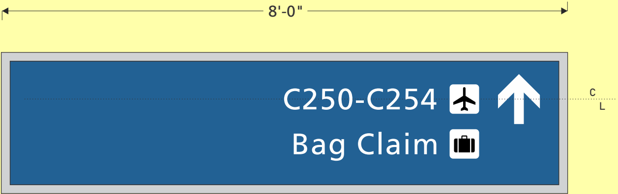
37 Graphic View (side A) Scale is 3/4" = 1'
