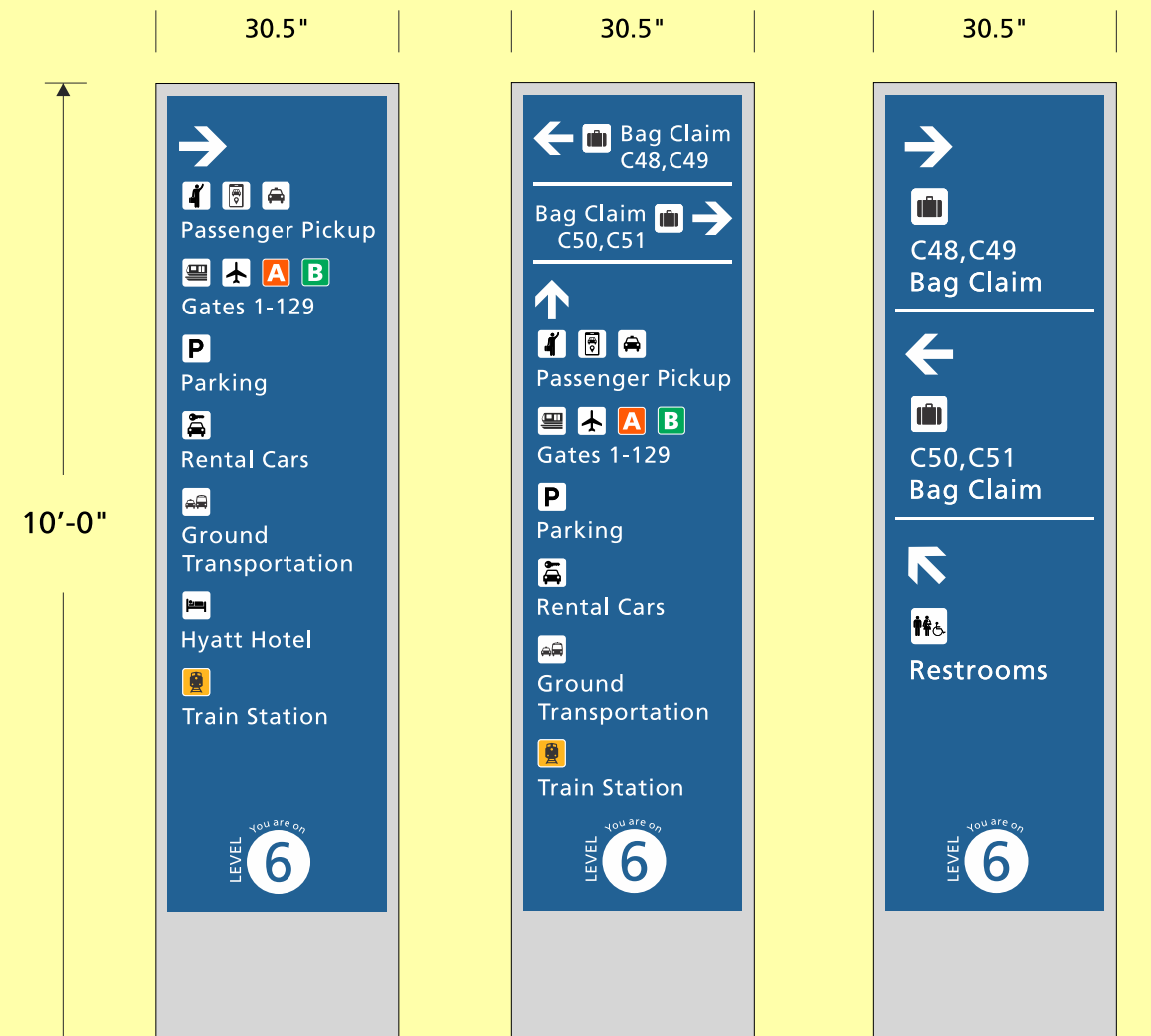
20.1 South Face View Scale is 1/2" = 1'
