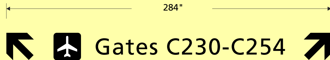
45.1 Concept Elevation Scale in 1/4" = 1'
