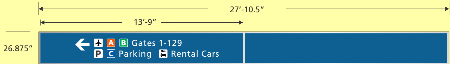
14 Existing View Scale is 1/4" = 1'
