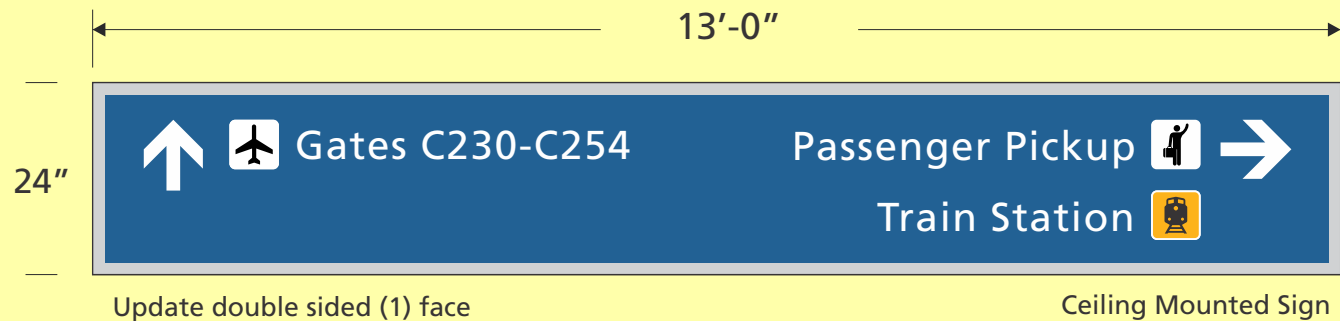
9 Proposed Graphic View (side A) Scale is 1/2" = 1'
