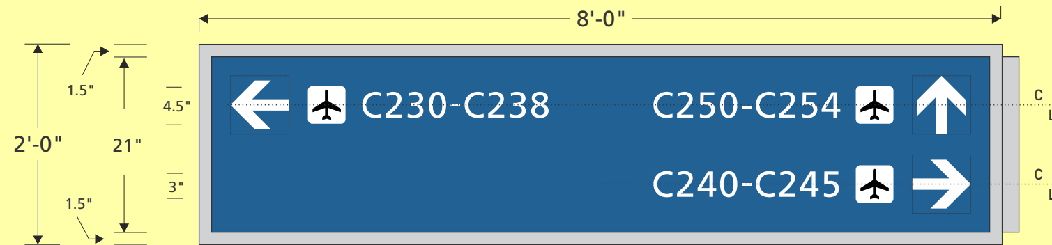
32 Graphic View (side B) Scale is 3/4" = 1'
