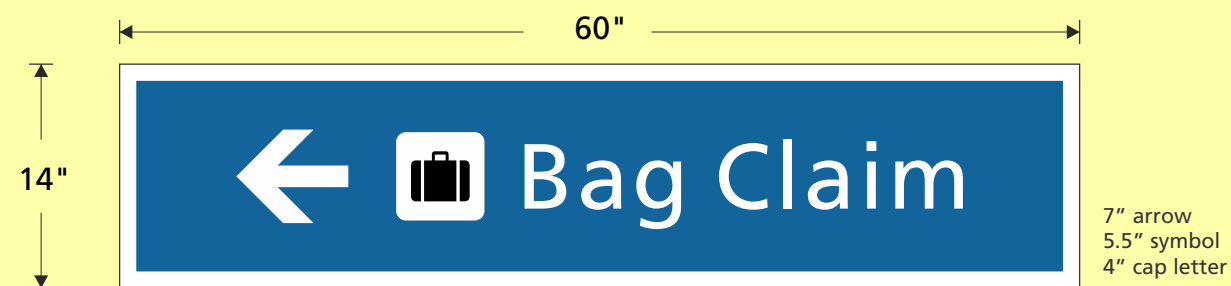
43.1 New Face View Scale is 1" = 1'
