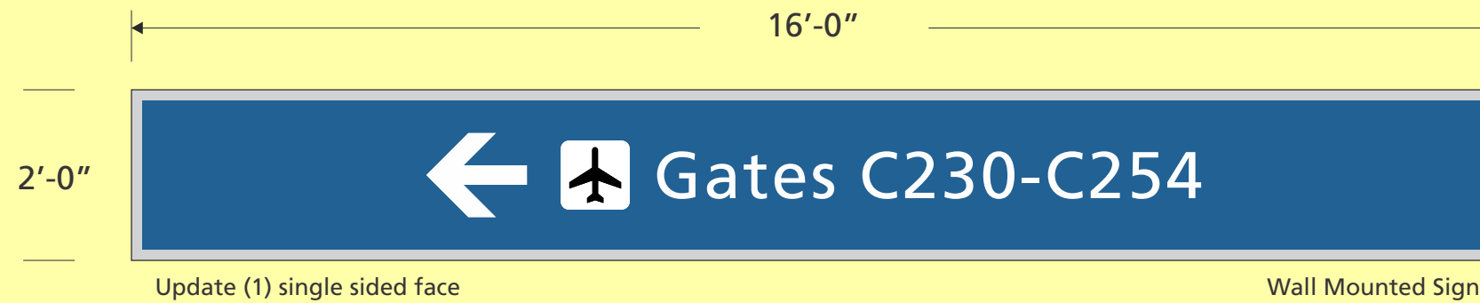
74 Graphic View Scale is 1/2" = 1'
