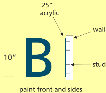
22.3 Side View Scale is 1" = 1'
