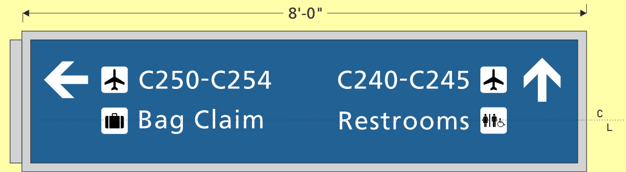
33 Graphic View (side B) Scale is 3/4" = 1'
