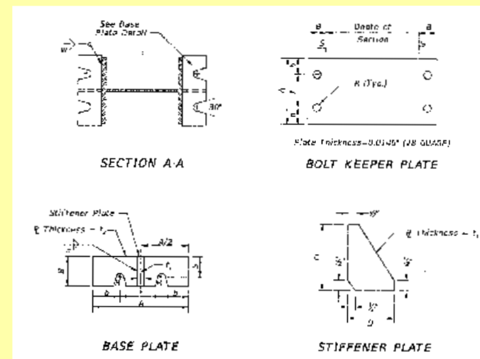
I-Beam - Plate & Stiffener
