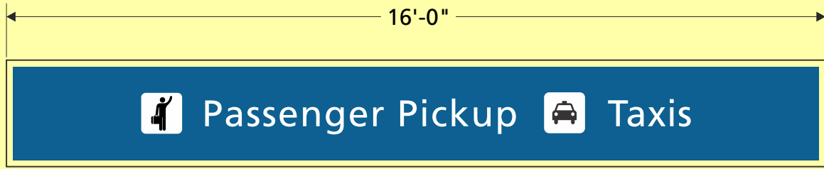
18.1 Graphic View (taxi assessable south exits) Scale is 3/8" = 1'
