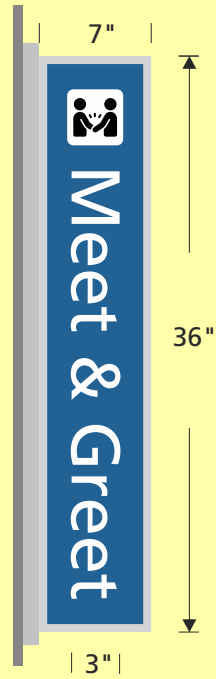
1.1 Graphic View Scale is 1" = 1'
