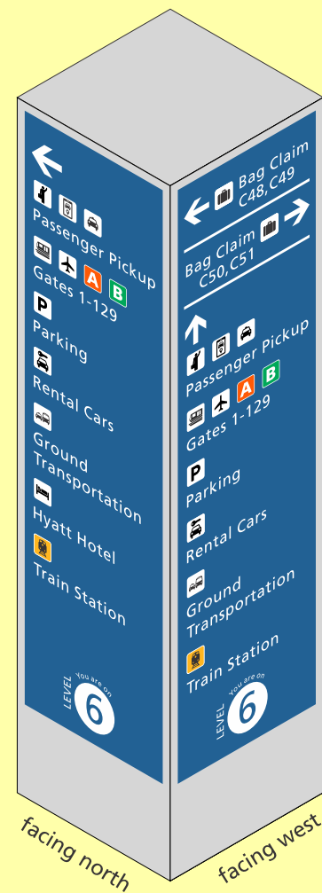
19.4 Side View Not to Scale
