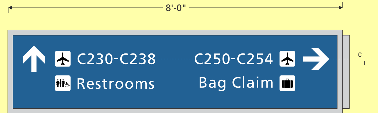
33 Graphic View (side A) Scale is 3/4" = 1'
