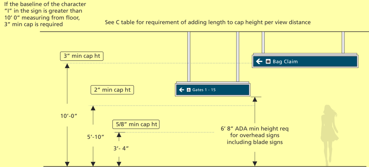
B ADA Mounting Heights Not to Scale
