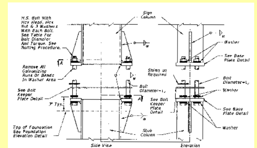
I-Beam - Base Connection
