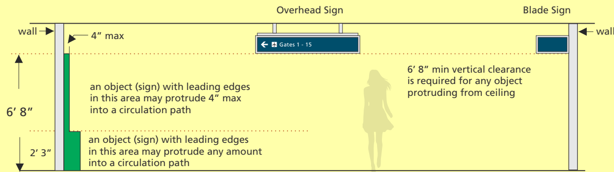
A ADA Protruding Conditions Not to Scale
