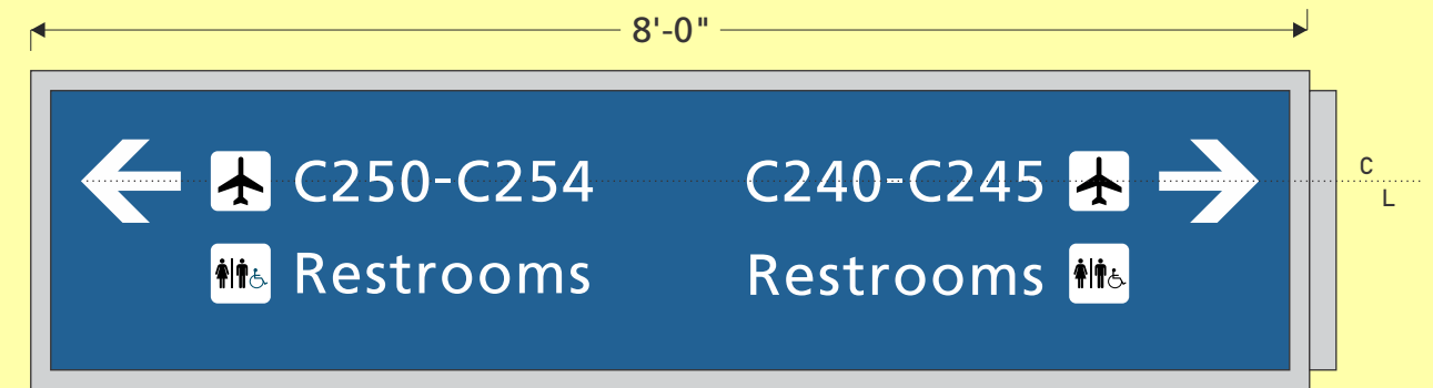
35 Graphic View (side B) Scale is 3/4" = 1'
