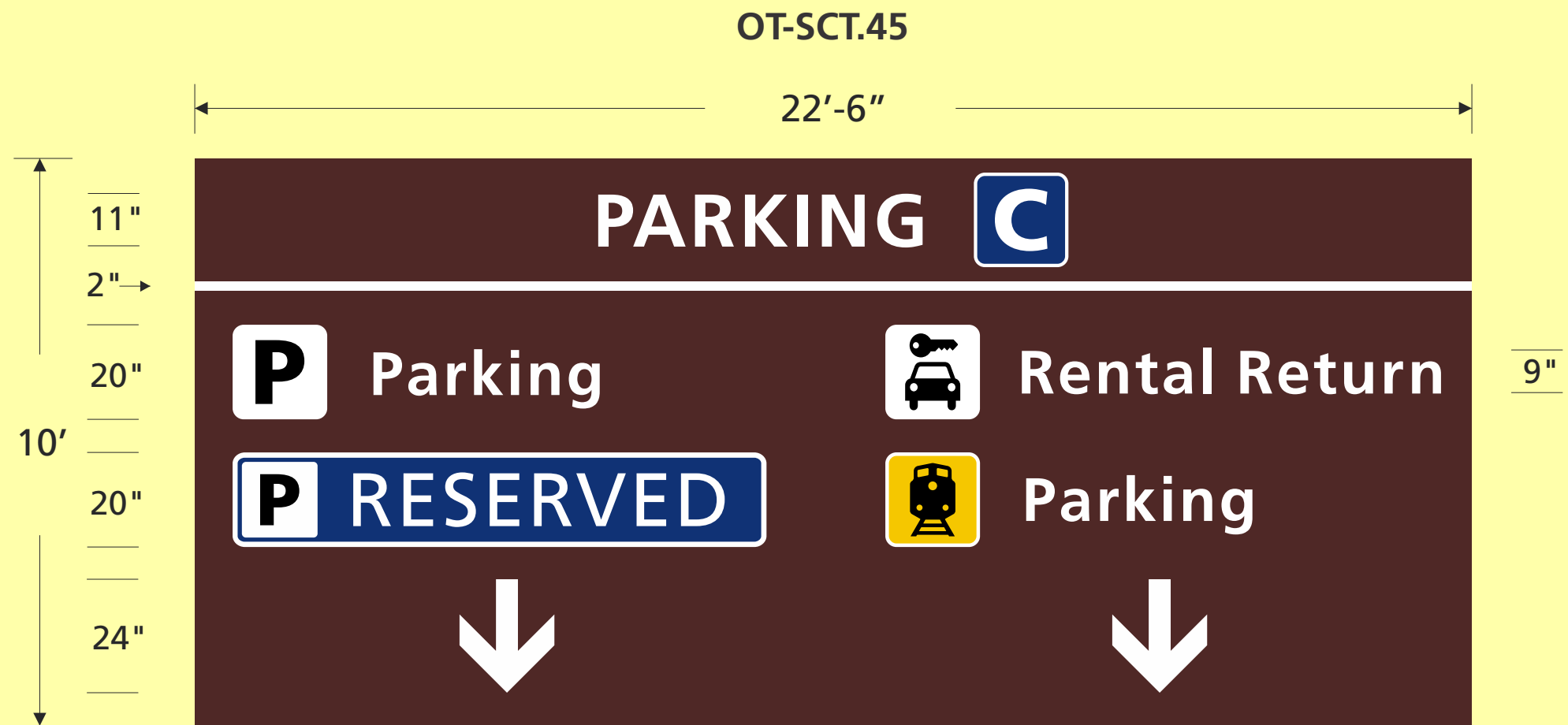
80 Graphic View Scale is 3/8" = 1'
