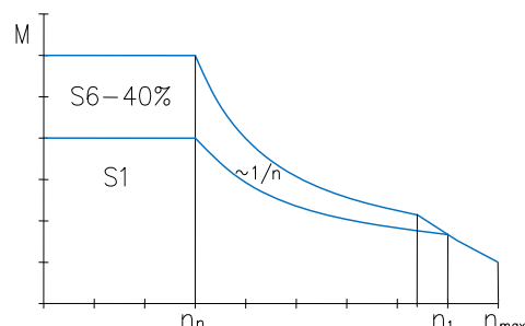
TORQUE DIAGRAM
