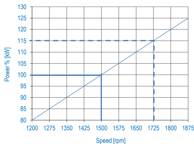
SPEED/POWER DIAGRAM
