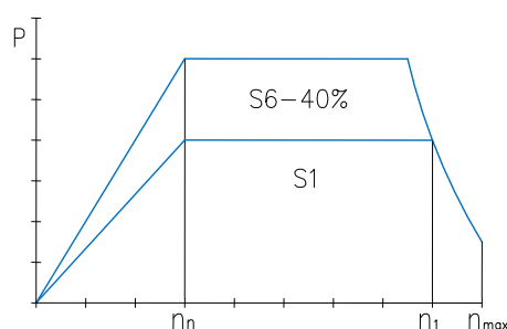
POWER DIAGRAM
