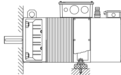
MONTAGGIO A FLANGIA + SUPPORTO MOUNTING WITH FLANGE + SUPPORT
