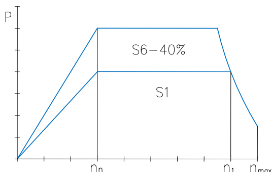
POWER DIAGRAM
