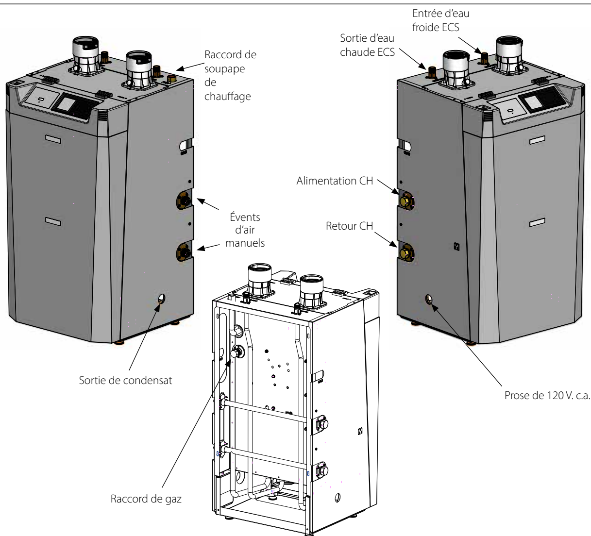
Fig. 19 - Instinct FSB Combi - Raccords de gaz/chauffage
