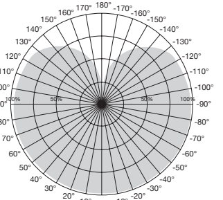
Beam Angle: 280° (Clear)
