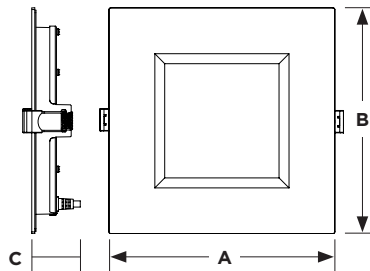
4" & 6" Adjustable Rough-In Mounting Plates
