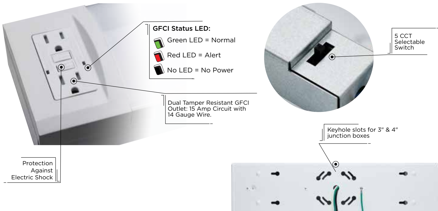
Rear Panel Mount
