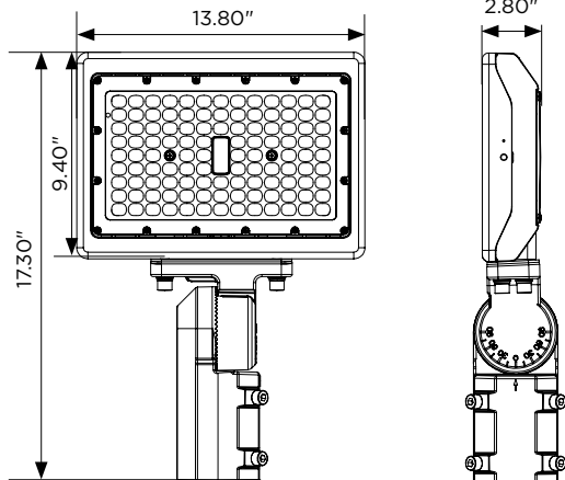
With slip-fitter mount
