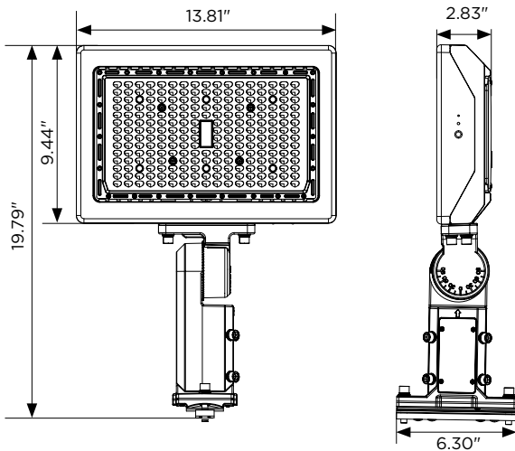
With universal mount
