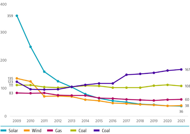
US unsubsidized cost of energy USD/MWh
