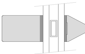
AVAILABLE IN 18MM OR 22MM GLASS SHOWN AS 14MM DOUBLE GLAZED UNIT
