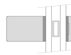
AVAILABLE IN 18MM OR 22MM GLASS SHOWN AS 14MM DOUBLE GLAZED UNIT
