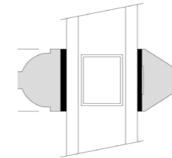
PROFILE AVAILABLE IN 18MM OR 22MM GLASS SHOWN AS 24MM DOUBLE GLAZED UNIT
