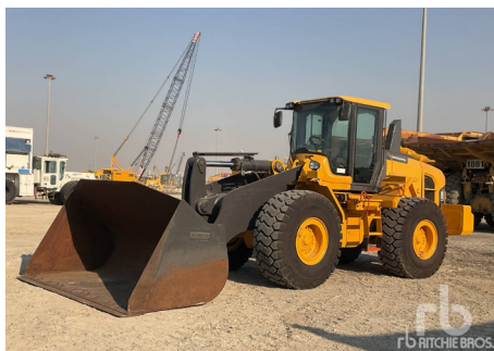
1 / 2, 2018 VOLVO L120GZ
