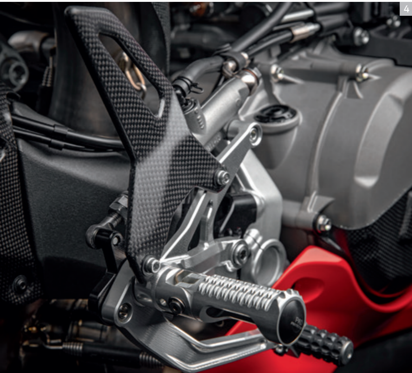
4 Carbon heel guard. Adjustable rider footpegs in aluminium.
