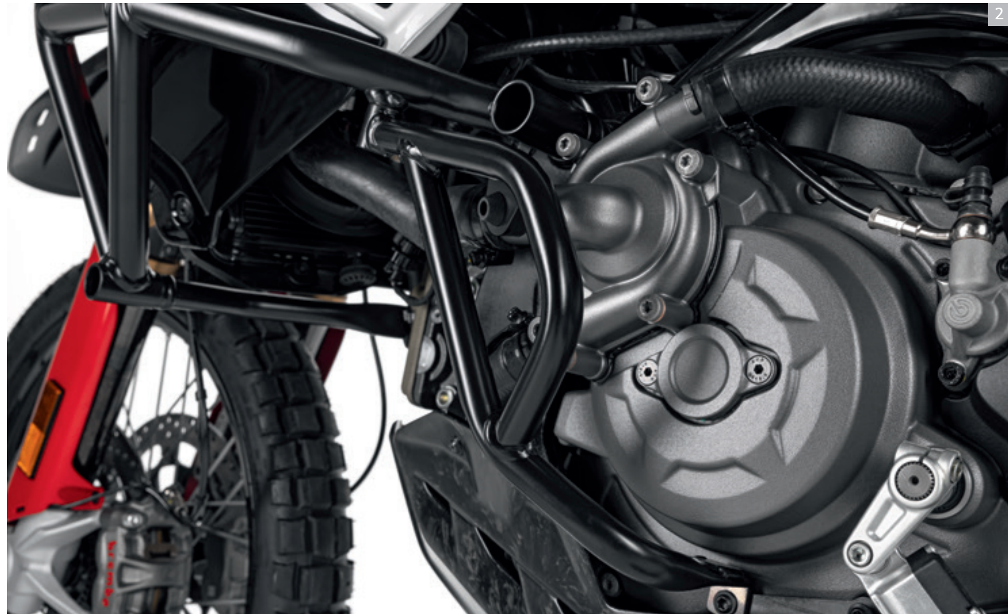
10 Water pump protection.
