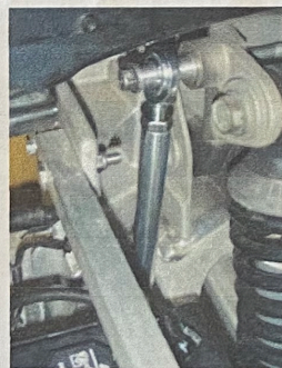
Figure 2 & 3 – Photos of the VSL's installed without rubber boots (for clarity)
