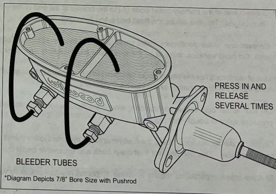
Typical Bleeder Tube Setup and Use
