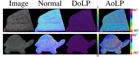
Figure 9: Qualitative results of our method on the objects with rough surfaces.
